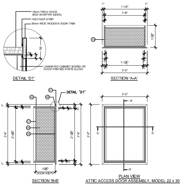
ATTIC ACCESS DOOR, MODEL 22 x 30 GENERAL ARRANGEMENT
