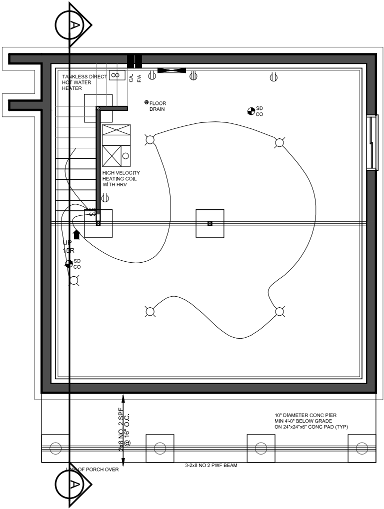
FOUNDATION PLAN SCALE: 3/16"=1'-0"
