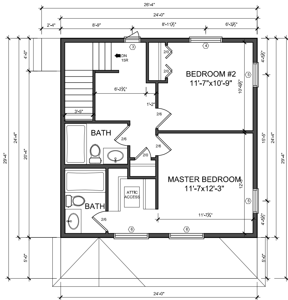
UPPER FLOOR PLAN SCALE: 3/16"=1'-0"
