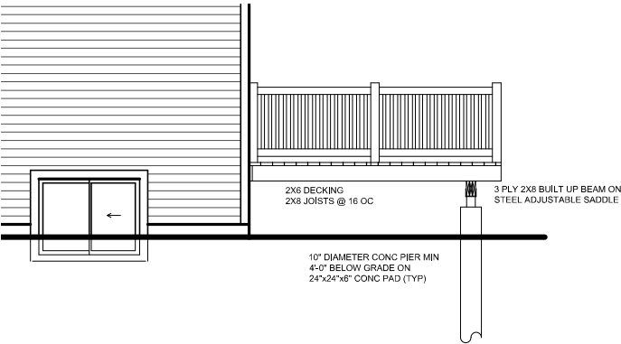
DECK SECTION SCALE: 3/16"=1'-0"
